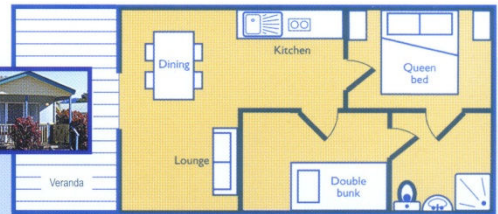
Hibiscus Villa (10m x 4.3m)
